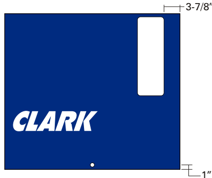
1CKWV1 42" (W) x 37-1/4" (H) x 1" (D) Wayne Vista Uni-hose (Full Height. No Totalizer Slots) Qty. _____ Pair
