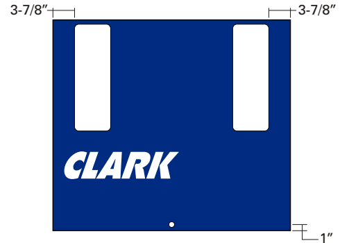
1CKWV2W4 42" (W) x 37-1/4" (H) x 1" (D) Wayne Vista 2-Hose (Full Height. No Totalizer Slots) Qty. _____ Pair
