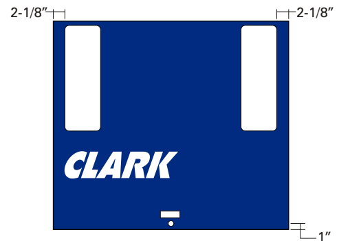
1CKWV2W2P 42" (W) x 37-1/4" (H) x 1" (D) Wayne Vista 2-Hose (Full Height. No Totalizer Slots. Pocket-Pull Handle) Qty. _____ Pair
