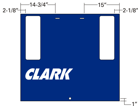
1CKWV2W2TC 42" (W) x 37-1/4" (H) x 1" (D) Wayne Vista 2-Hose (Full Height. Totalizer Slots) Qty. _____ Pair
