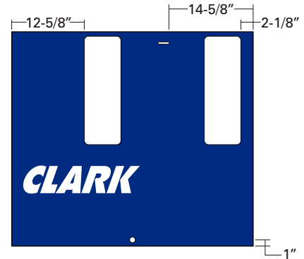
1CKWV2TC 42" (W) x 37-1/4" (H) x 1" (D) Wayne Vista 2-Hose (Full Height. Totalizer Slots) Qty. _____ Pair
