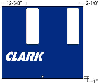
1CKWV2 42" (W) x 37-1/4" (H) x 1" (D) Wayne Vista 2-Hose (Full Height. No Totalizer Slots) Qty. _____ Pair
